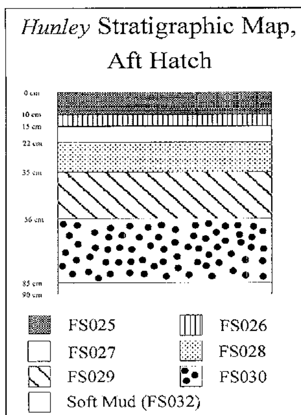
Figure 9.7. Stratigraphic profile.
