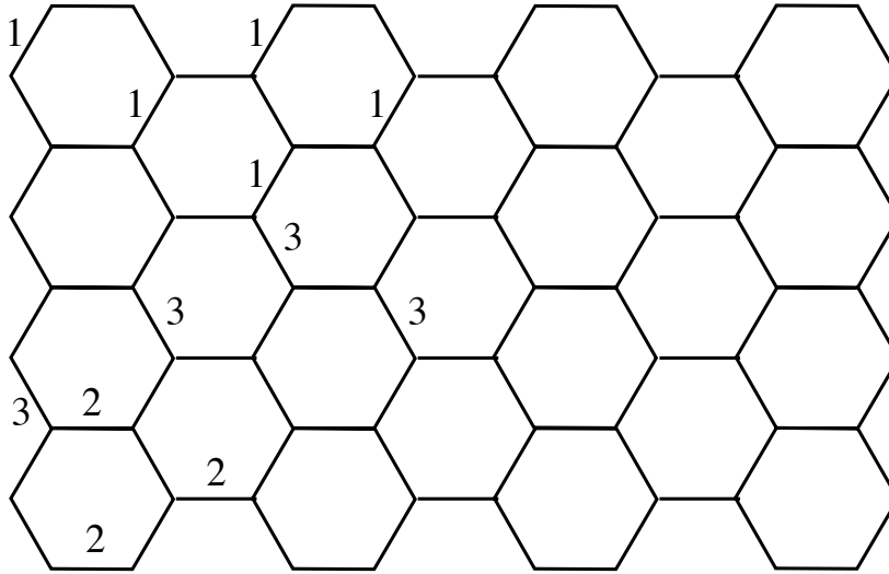
Figure 3: Hexagonal lattice
