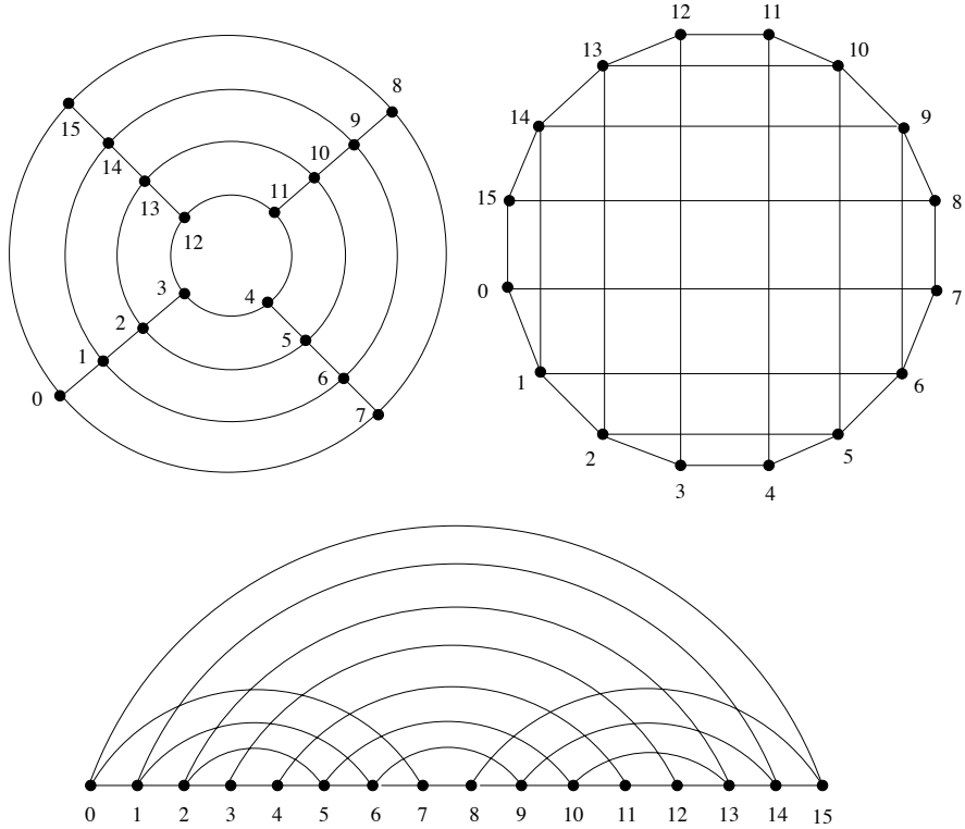
Figure 1: The 4 \times 4 cylindrical grid and its convex and one-page drawings
