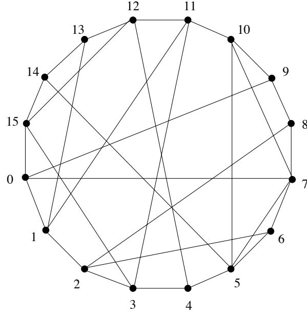
Figure 2: A convex drawing of a 16-vertex graph. E.g. the distance of 0 and 9 is 7.
