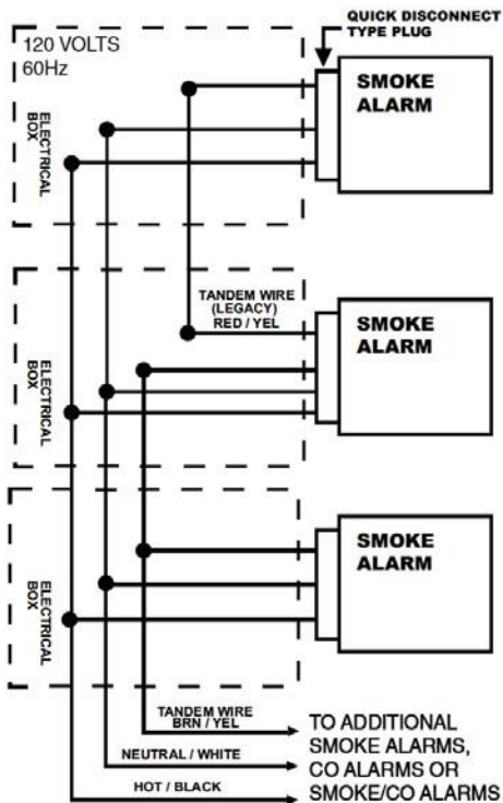
Tandem Wiring Diagram
