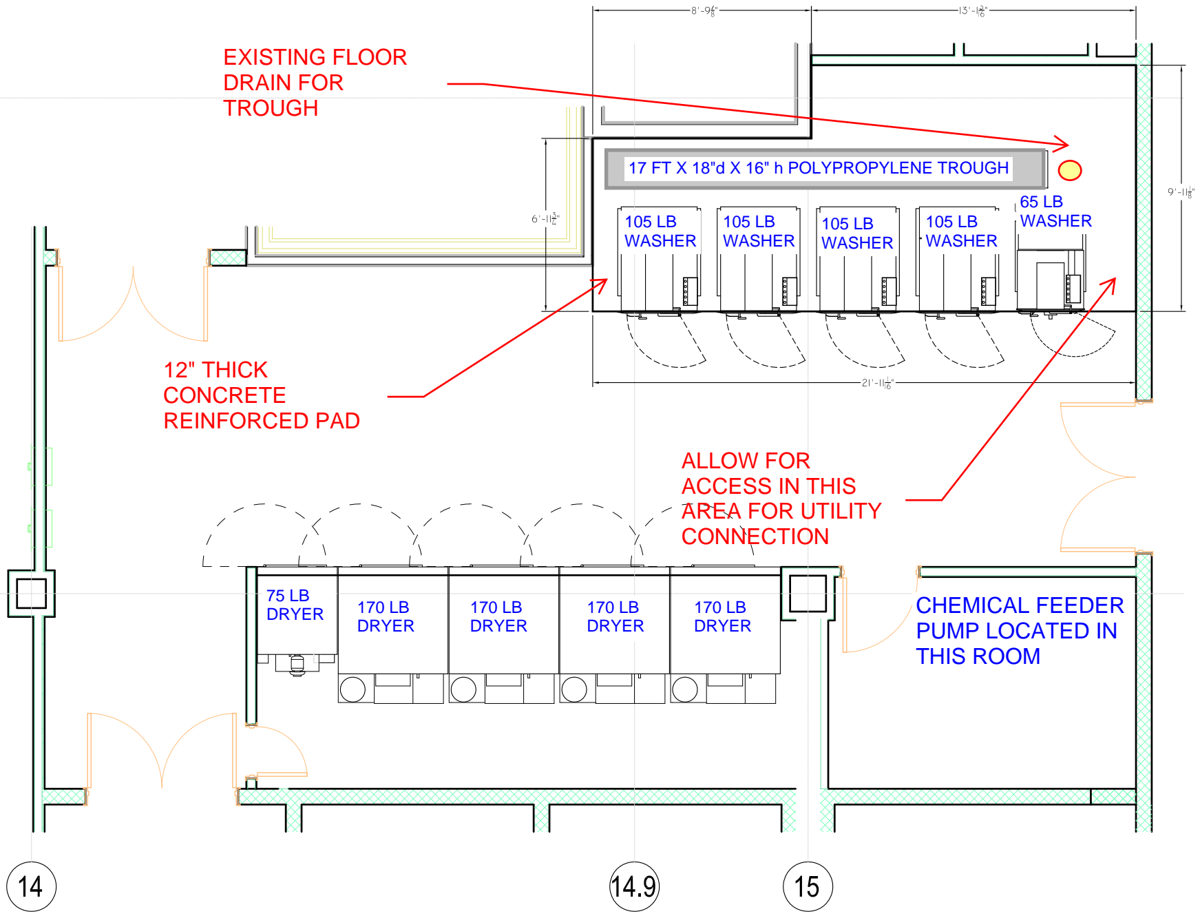
USC FOOTBALL OPERATIONS CENTER LAUNDRY ROOM FLOOR PLAN
