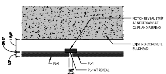
3 REVEAL DETAIL 1/16" = 1'-0"
