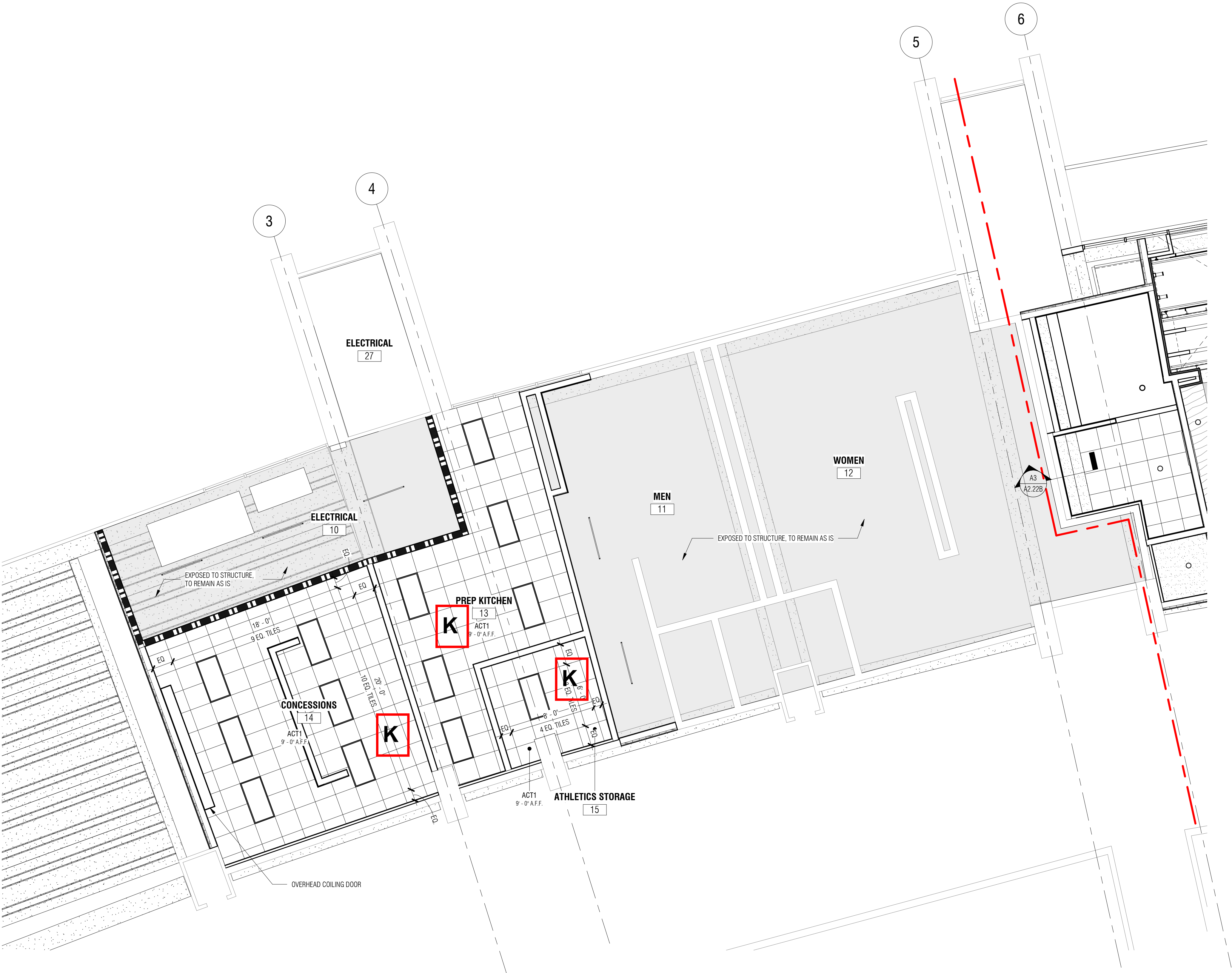
A1 A2.01A LEVEL 100 RCP 3/16" = 1'-0"
