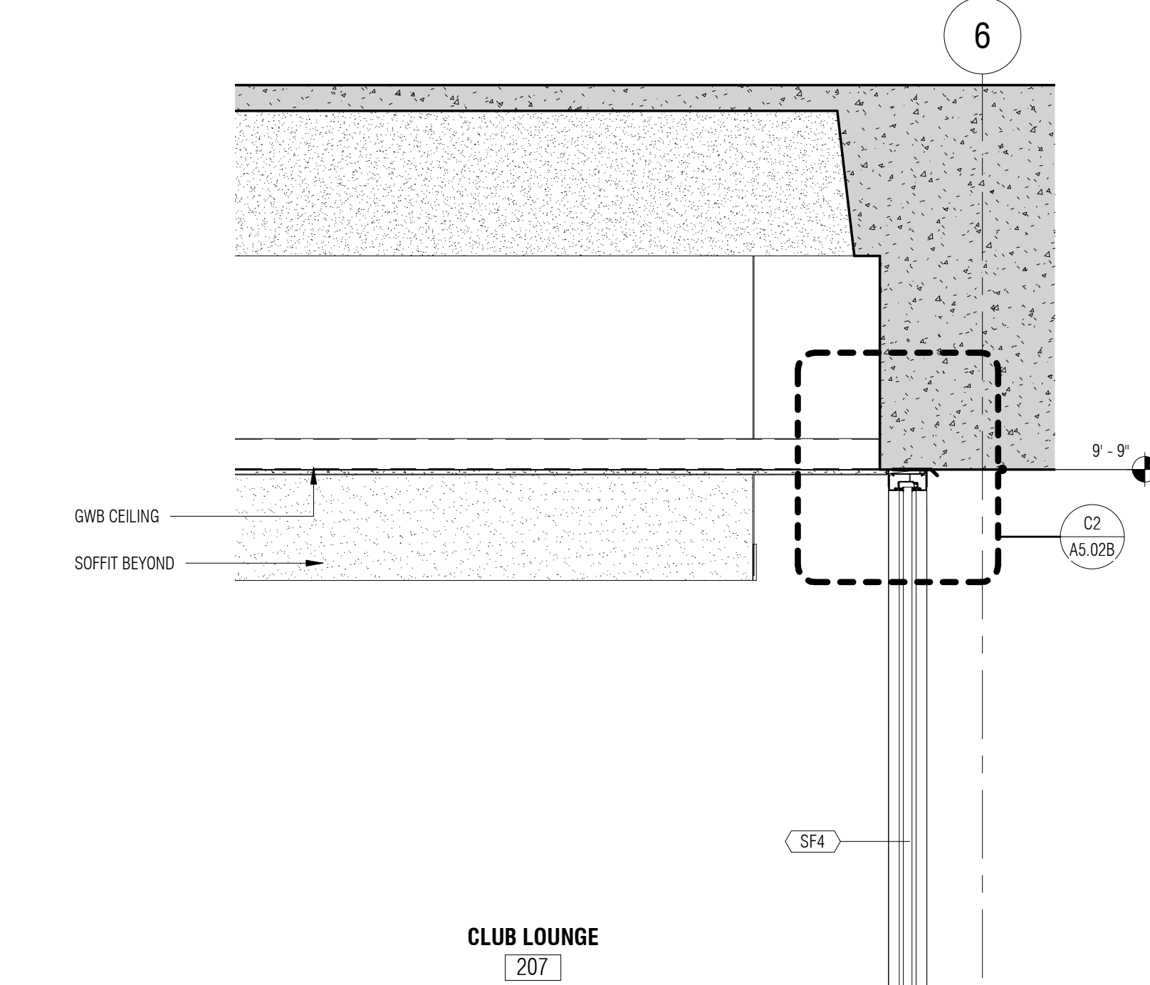
E4 JAMB DETAIL A5.02B 1 1/2" = 1'-0"
