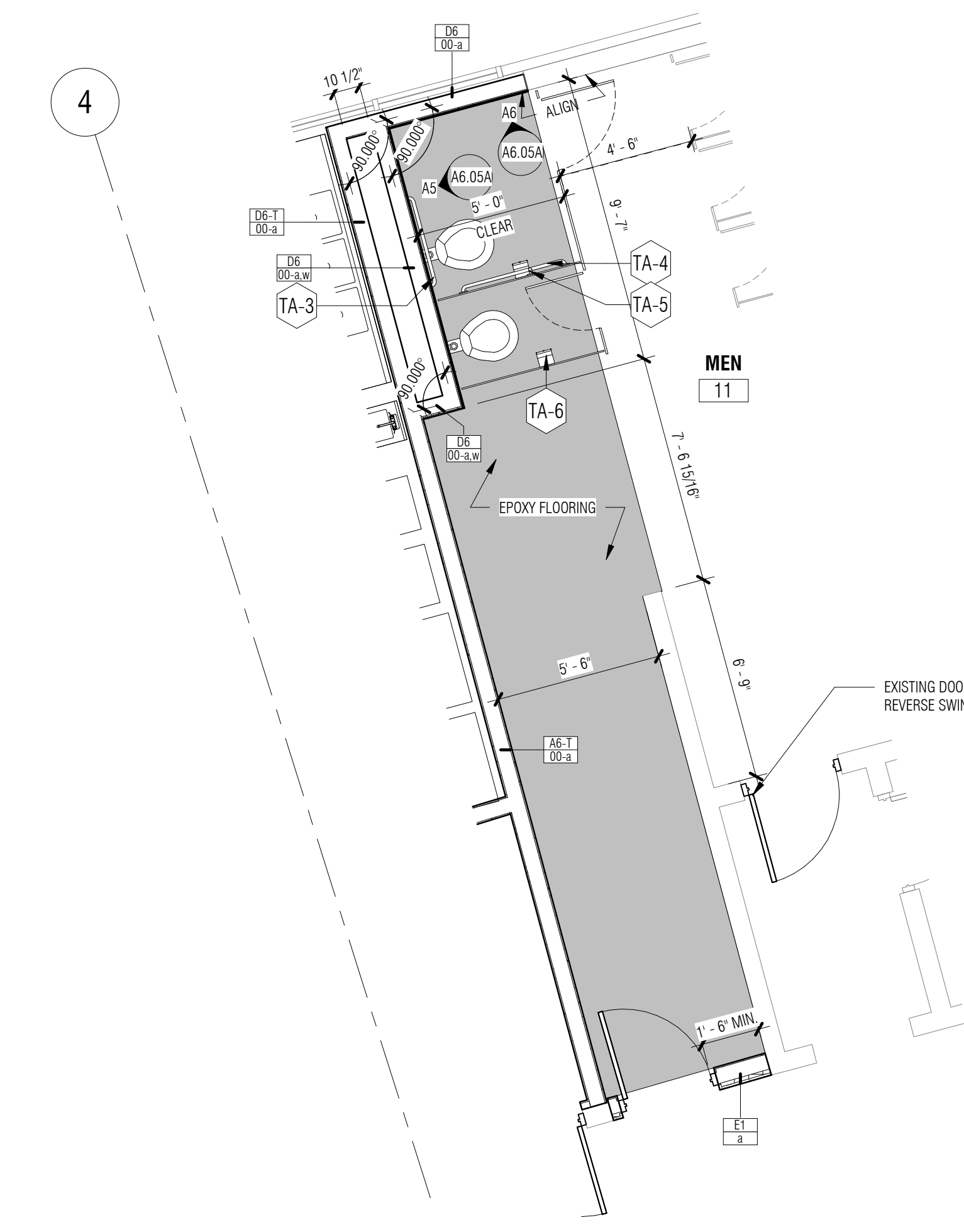
B5 LEVEL 100 MEN'S PUBLIC RESTROOM A6.05A 1/4" = 1'-0"
