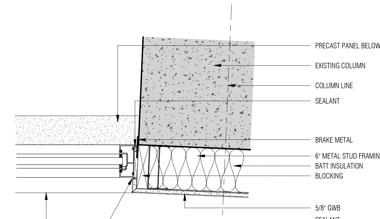
E4 JAMB DETAIL A5.02B 1 1/2" = 1'-0"
