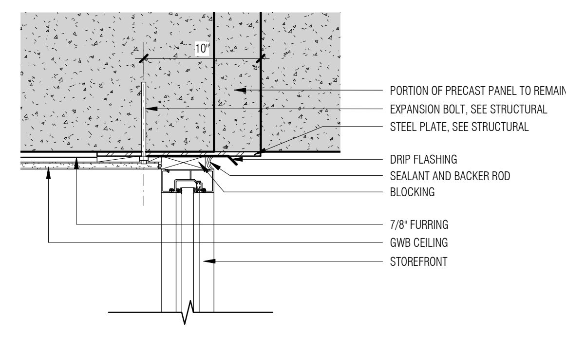
E1 SF HEAD DETAIL A5.02B 1 1/2" = 1'-0"
