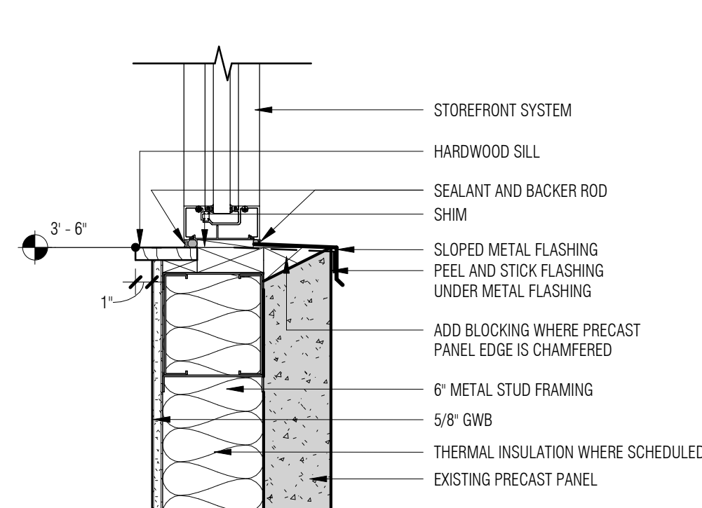
E2 SF SILL DETAIL A5.02B 1 1/2" = 1'-0"
