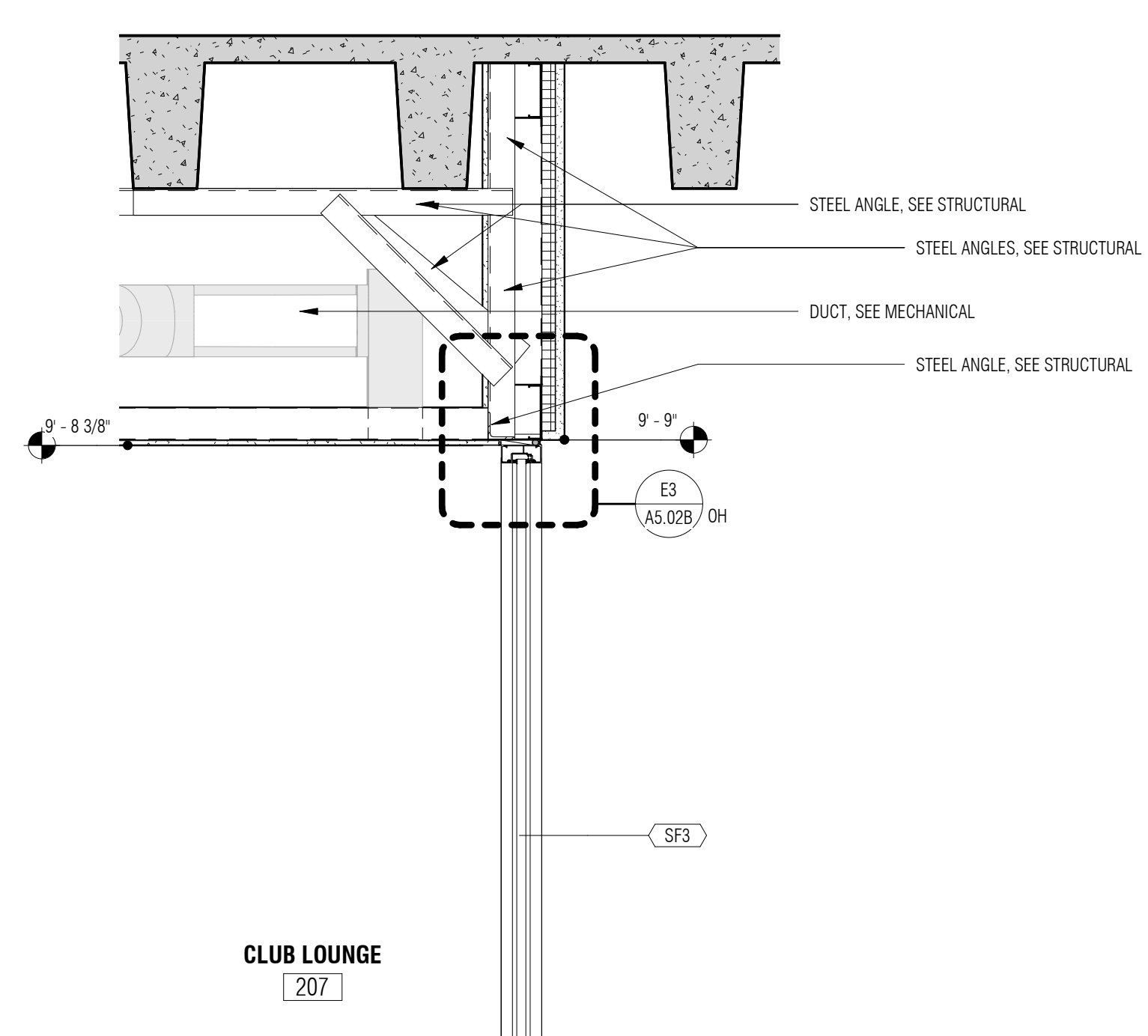
E6 SF JAMB DETAIL A5.02B 1 1/2" = 1'-0"
