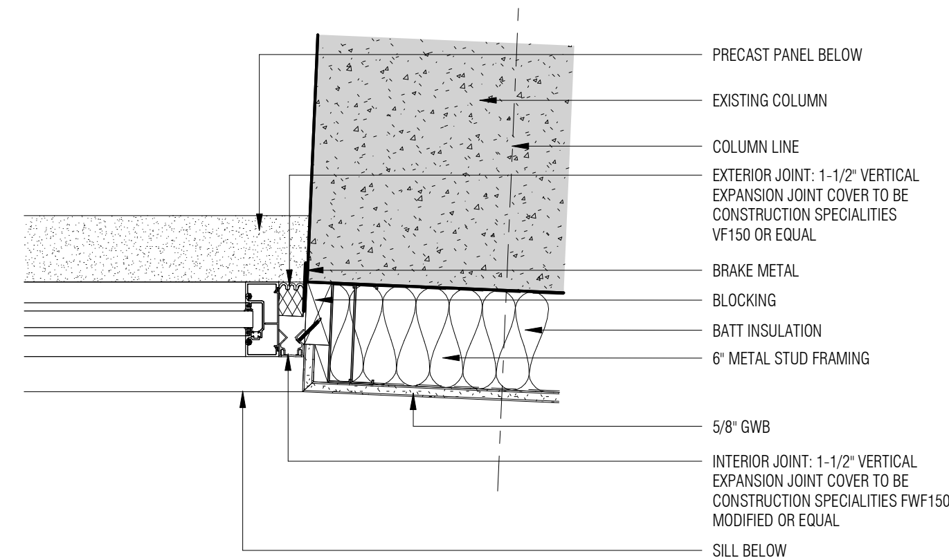
C3 SF JAMB DETAIL A5.02B 1 1/2" = 1'-0"
