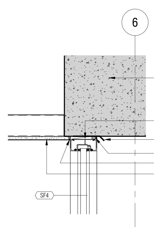
C2 SF HEAD DETAIL A5.02B 1 1/2" = 1'-0"
