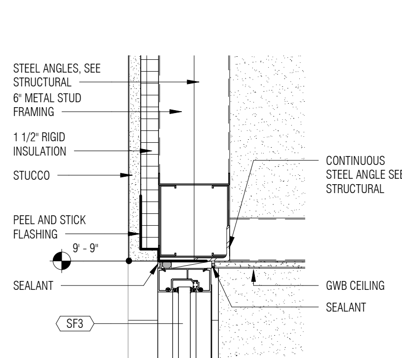
E3 SF HEAD DETAIL A5.02B 1 1/2" = 1'-0"
