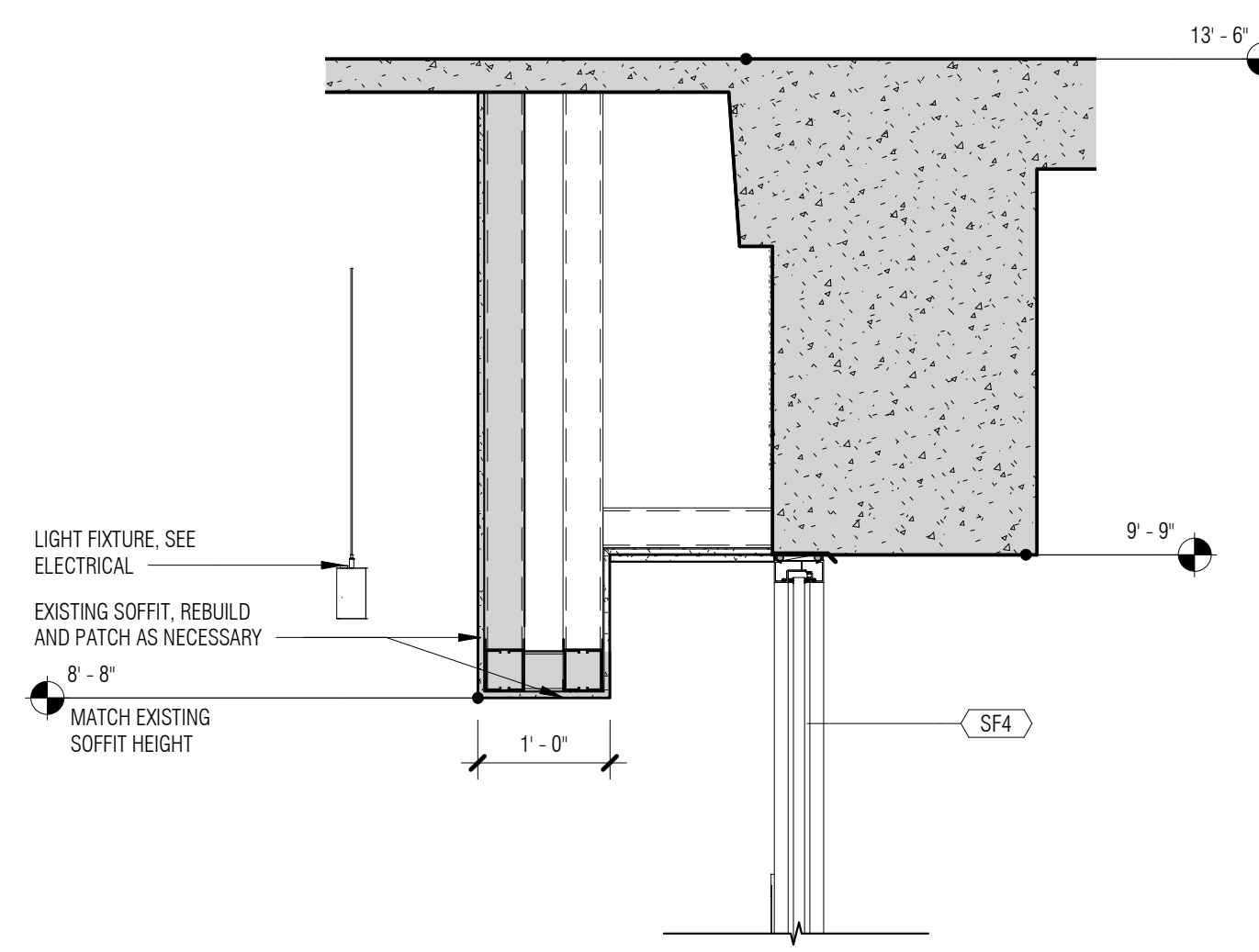
A2 CEILING DETAIL A5.02B 3/4" = 1'-0"
