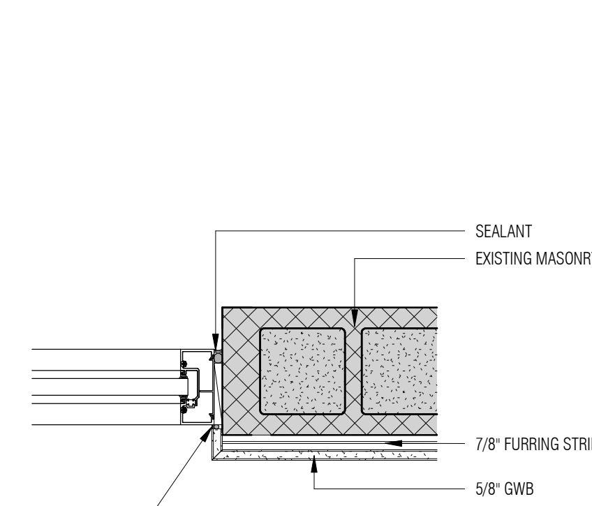
E5 SF JAMB DETAIL A5.02B 1 1/2" = 1'-0"
