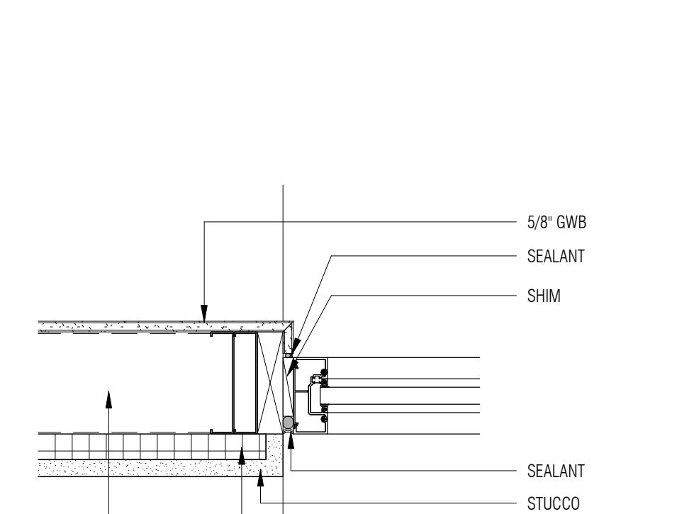
E6 SF JAMB DETAIL A5.02B 1 1/2" = 1'-0"
