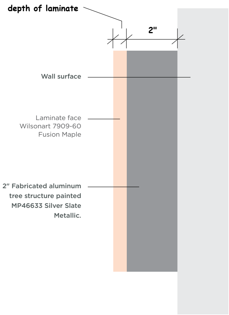
DETAIL VIEW : MILLWORK TREE, SIDE
