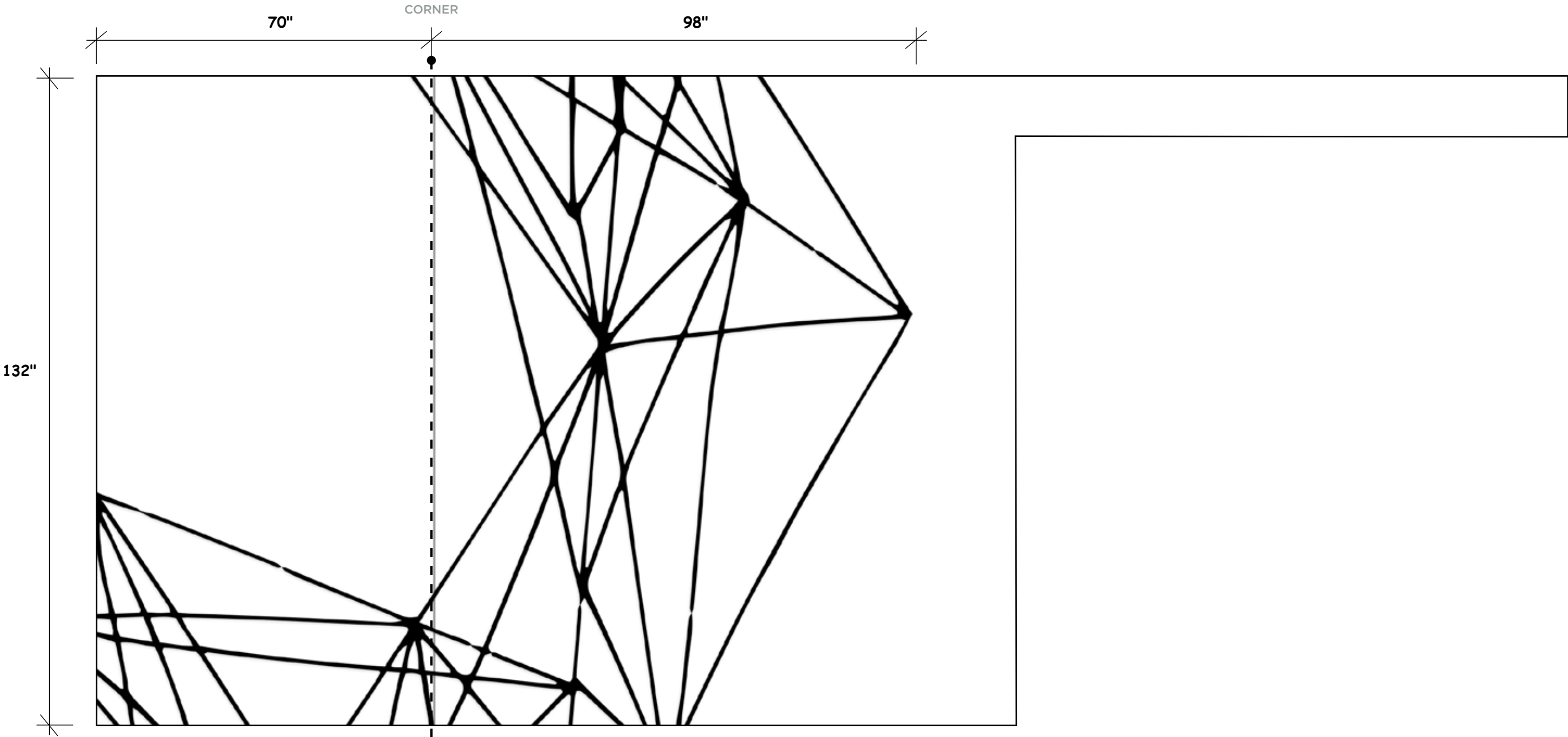
DETAIL VIEW: LAMINATE WALL PATTERN SHOWN BLACK FOR VISIBILITY (measurements shown include molding). Abet Laminait 3607 Diafos Sei Due laminate applied to 1/4" substrate with white returns.
