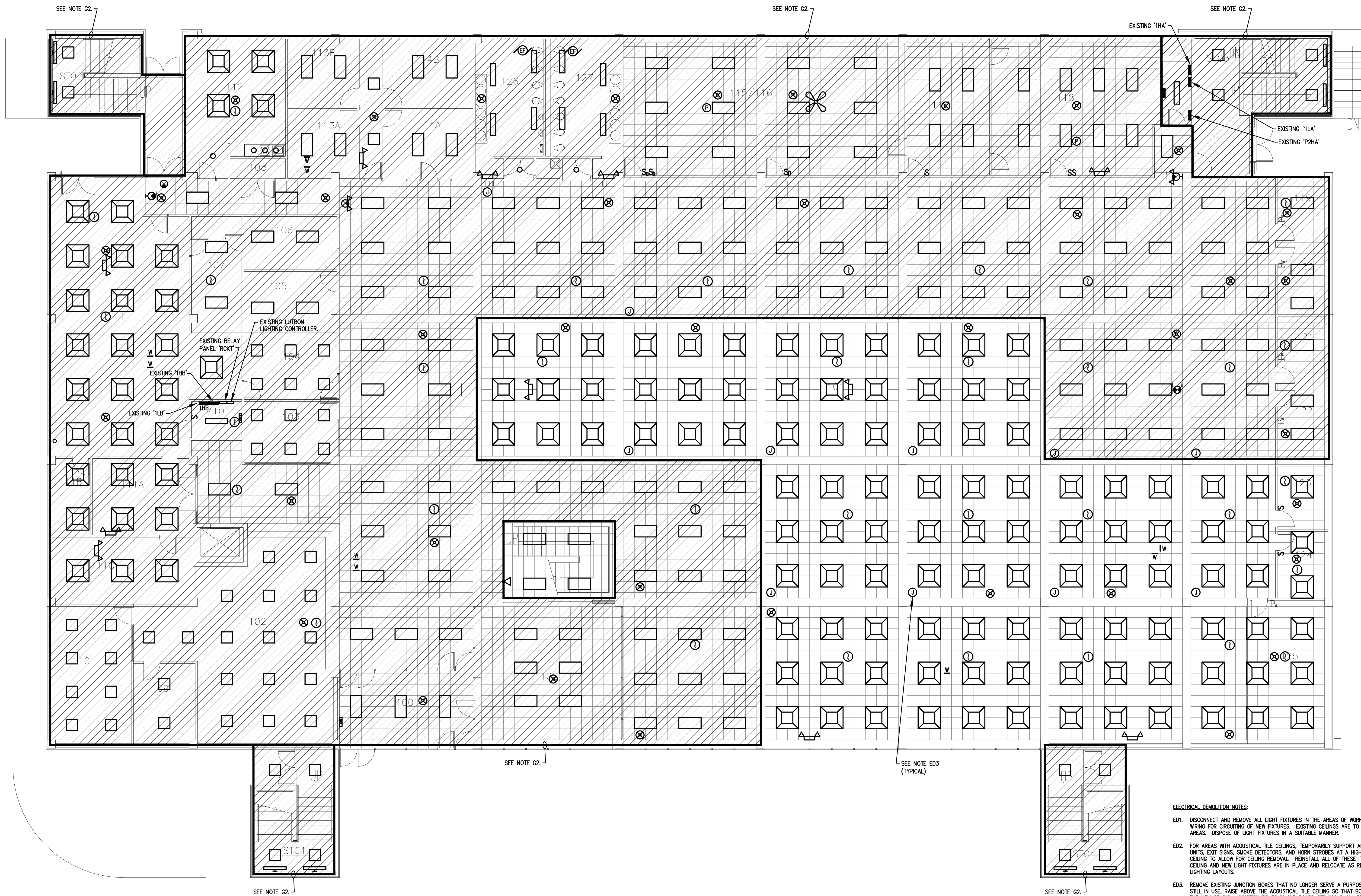
A ELECTRICAL DEMOLITION PLAN - 1st FLOOR ED1.1 SCALE: 1/8" = 1'-0"
