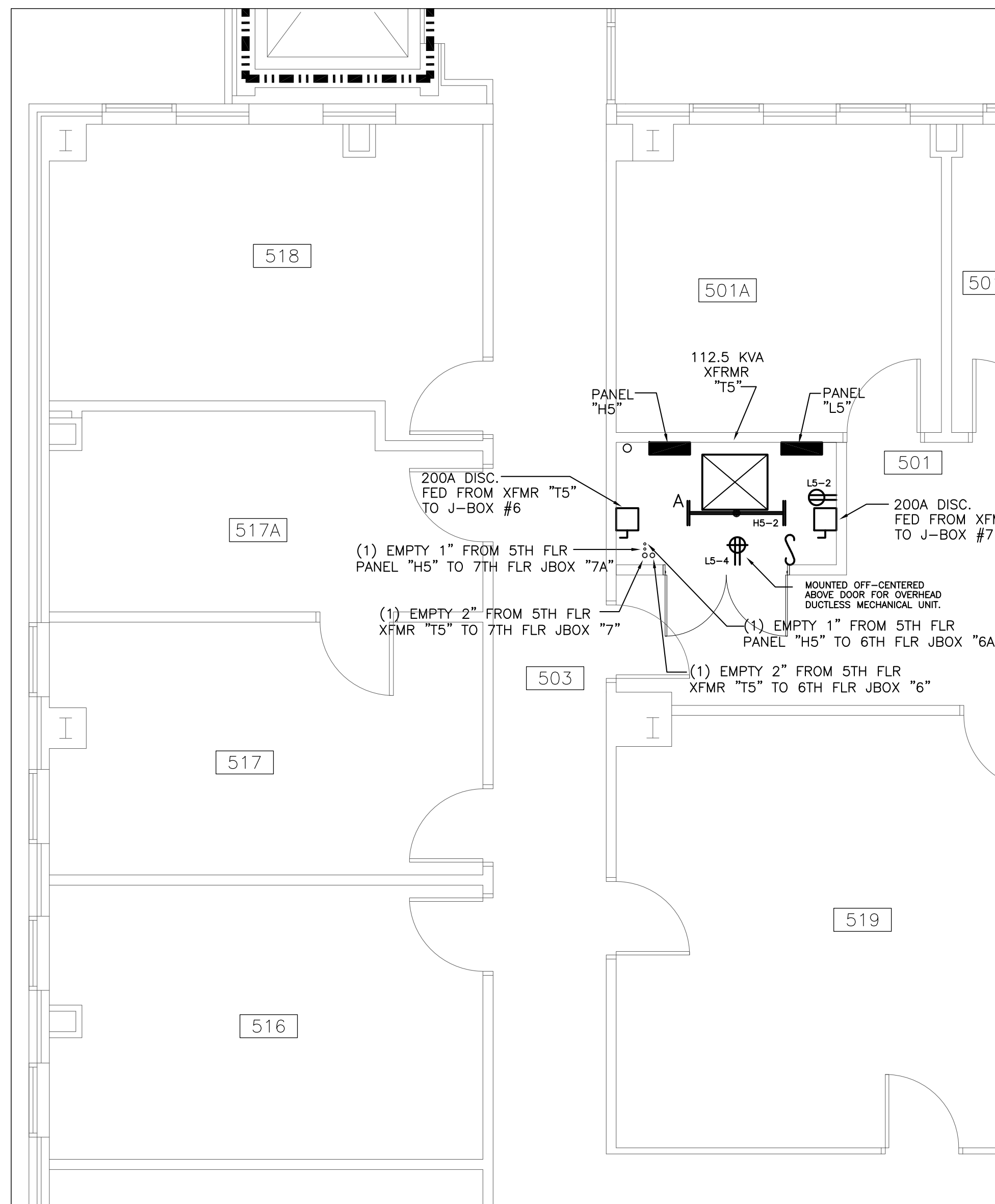
4 E4 5TH FLOOR ELECTRICAL RM. SCALE: 1/4" = 1'-0"
