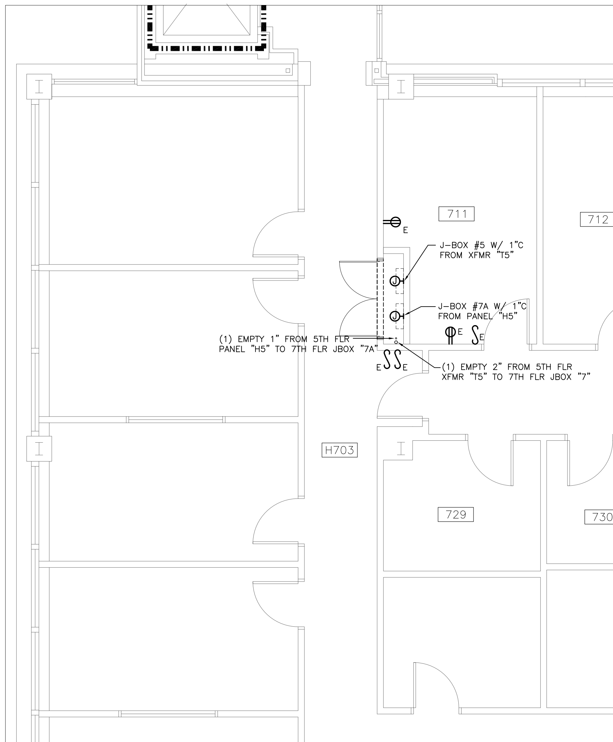
6 E4 7TH FLOOR ELECTRICAL RM. SCALE: 1/4" = 1'-0"
