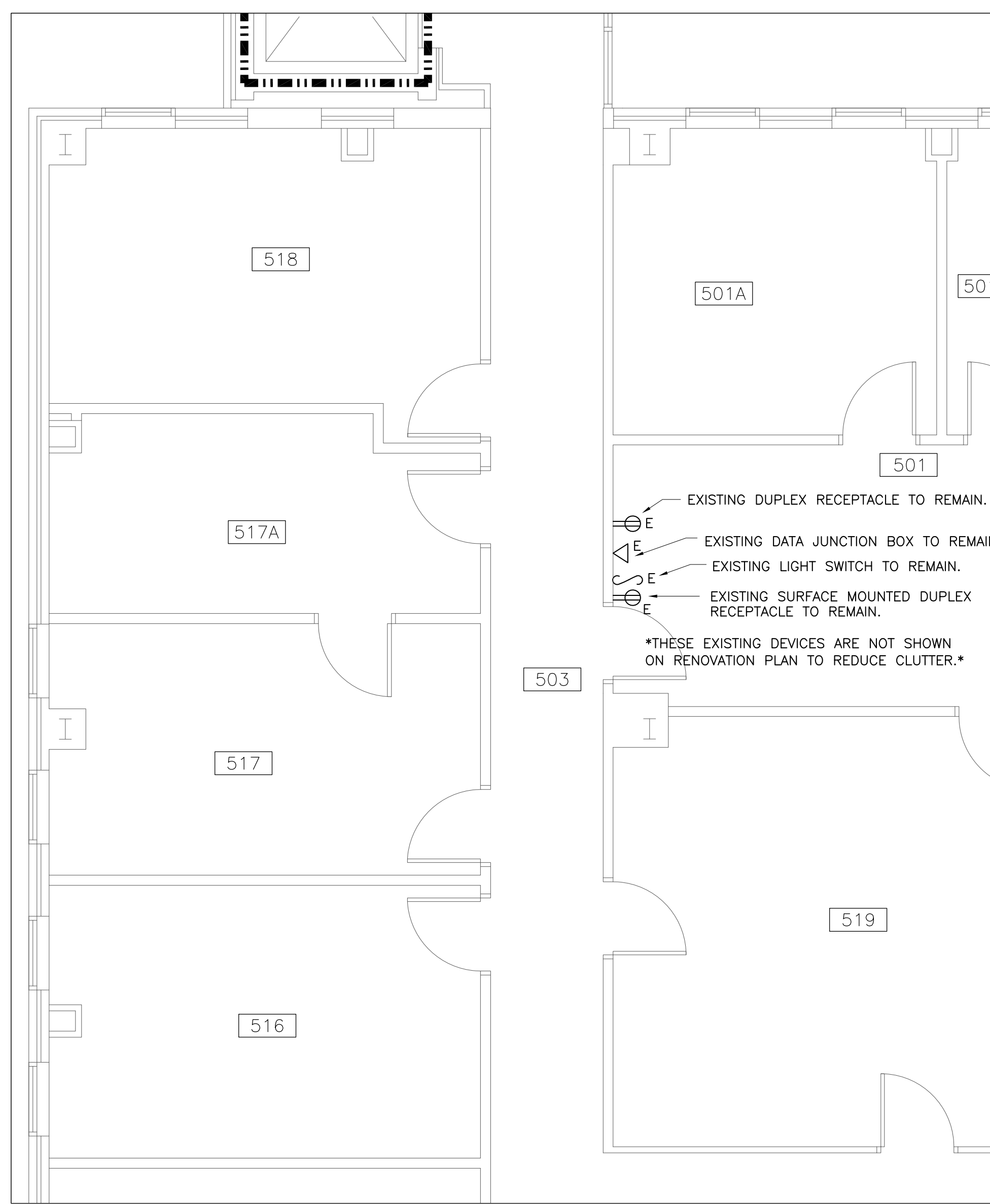
1 E4 5TH FLOOR PARTIAL DEMOLITION PLAN SCALE: 1/4" = 1'-0"
