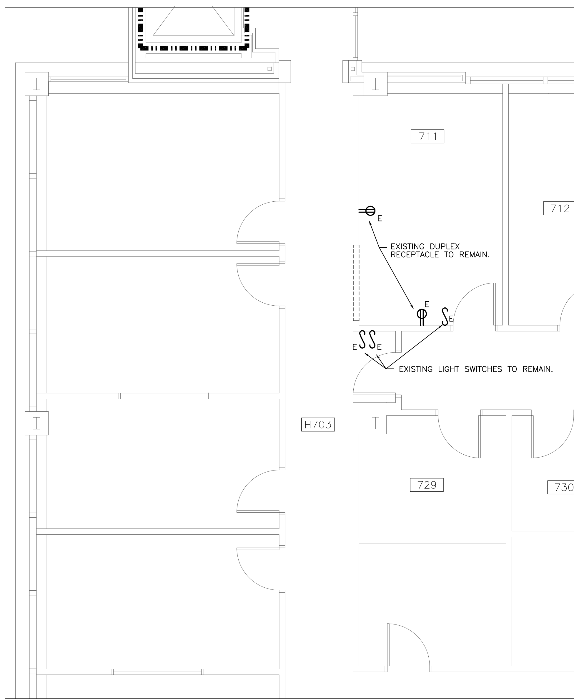
3 E4 7TH FLOOR PARTIAL DEMOLITION PLAN SCALE: 1/4" = 1'-0"
