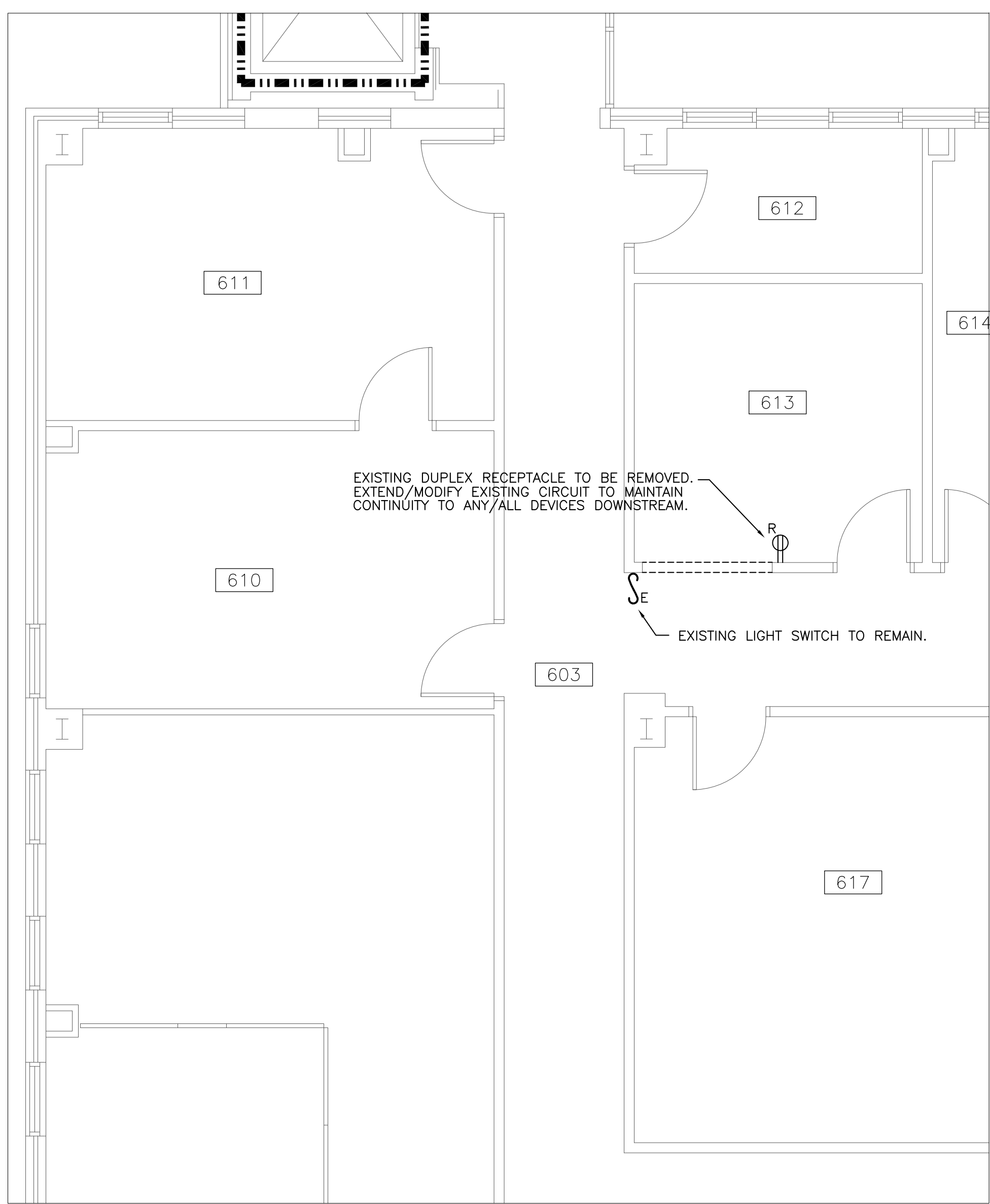
2 E4 6TH FLOOR PARTIAL DEMOLITION PLAN SCALE: 1/4" = 1'-0"
