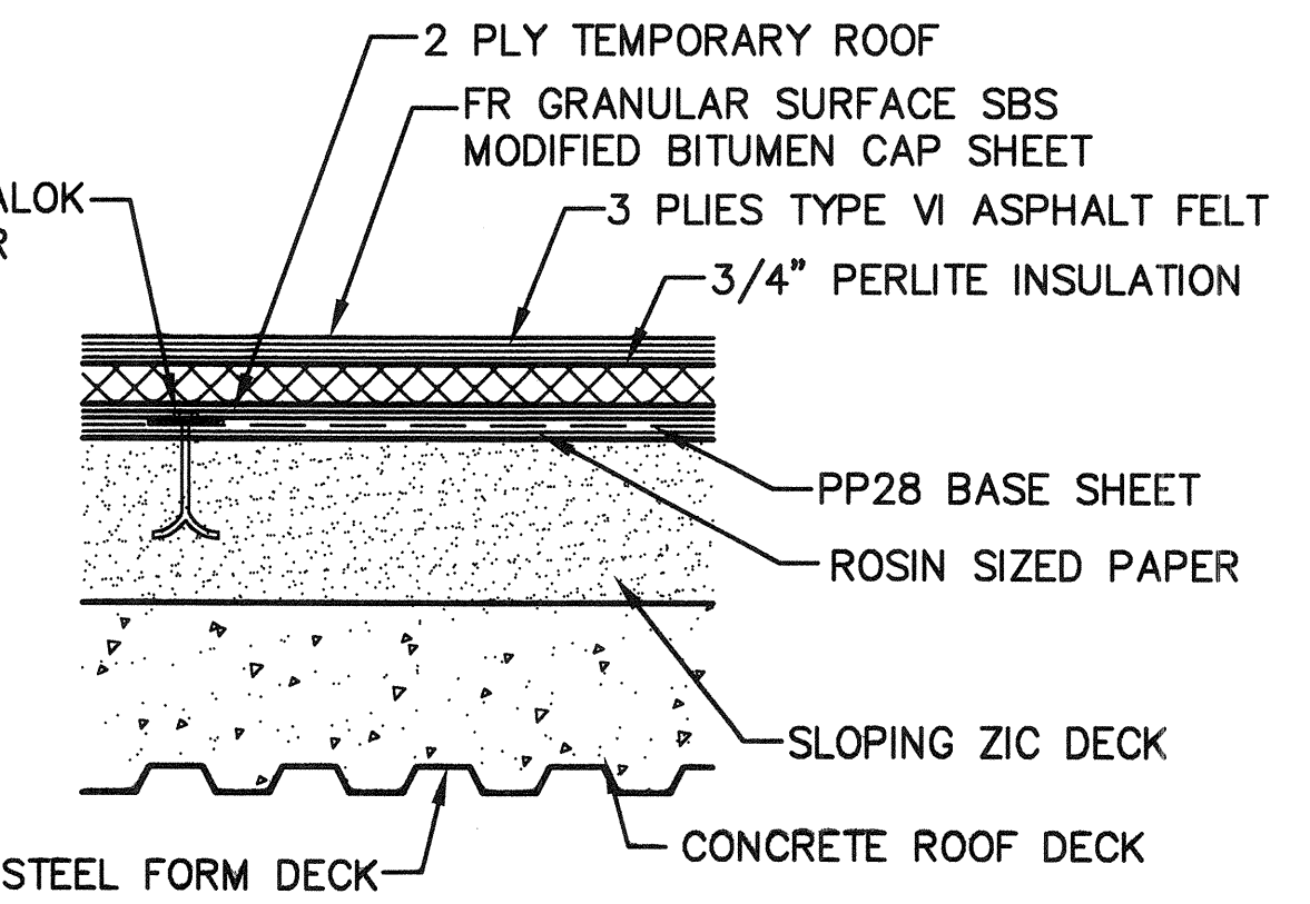
TYPICAL ROOF "D" ASSEMBLY NTS
