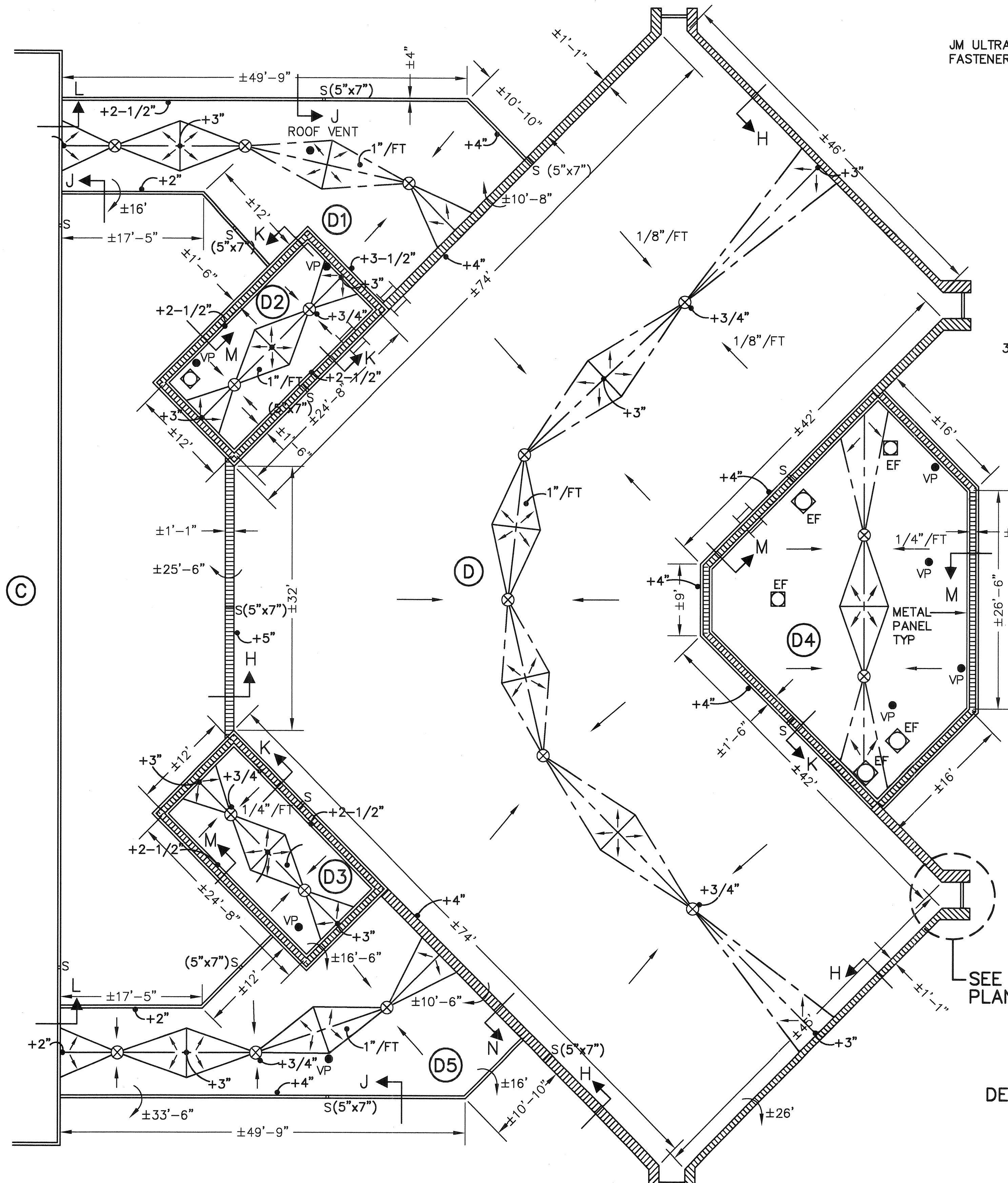
NEW ROOF PLAN - AREA D SCALE: 1/8"=1'-0"
