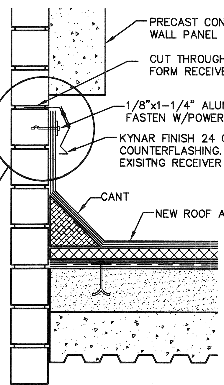
SECTION K-K NTS
