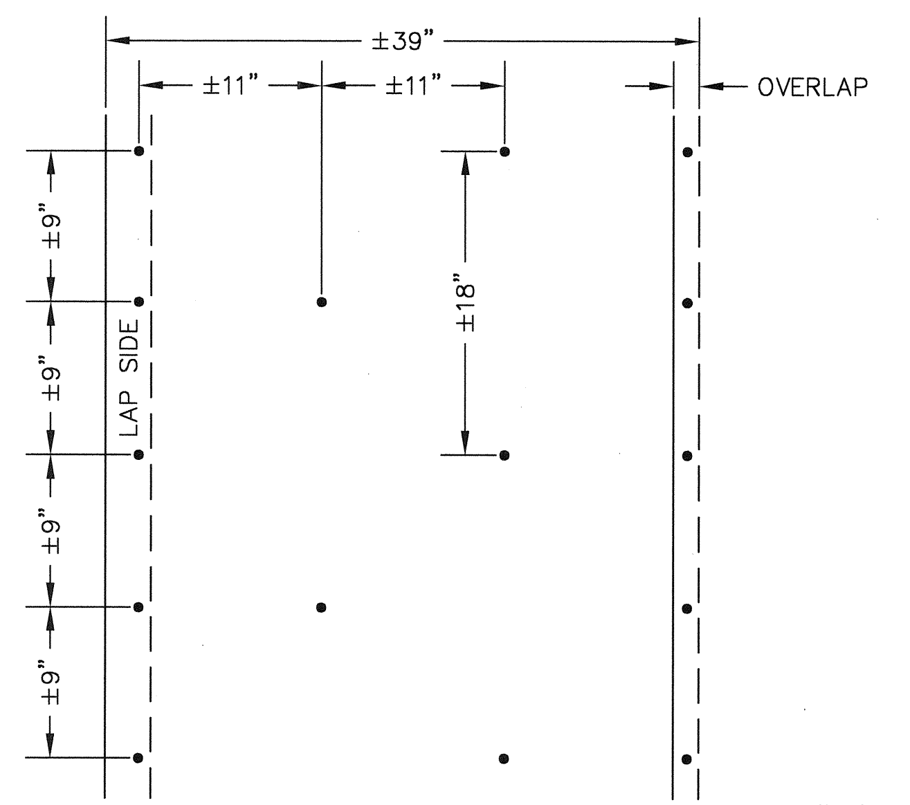
BASE SHEET FASTENER PATTERN AREA "D" NTS
