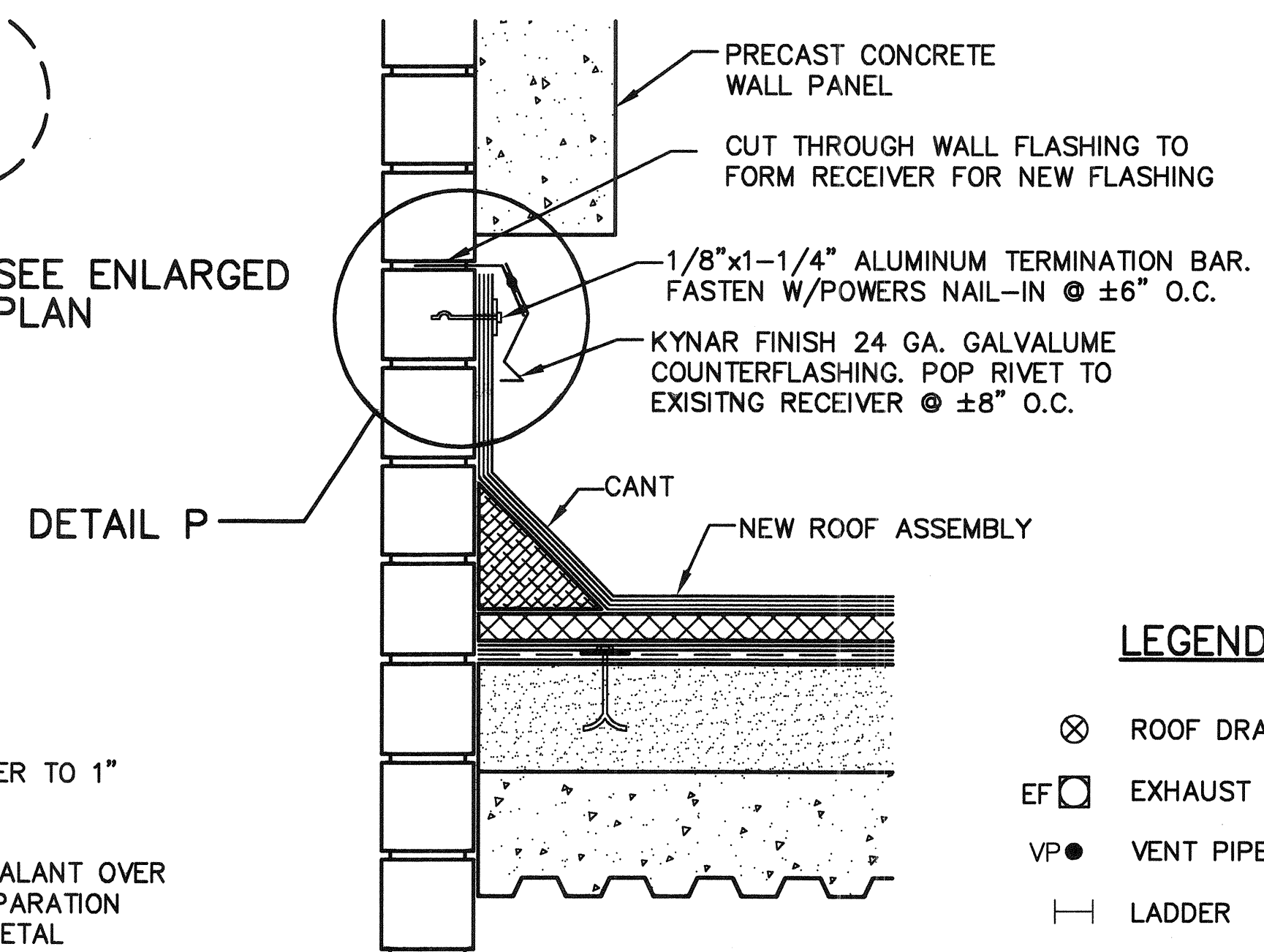
SECTION K-K NTS
