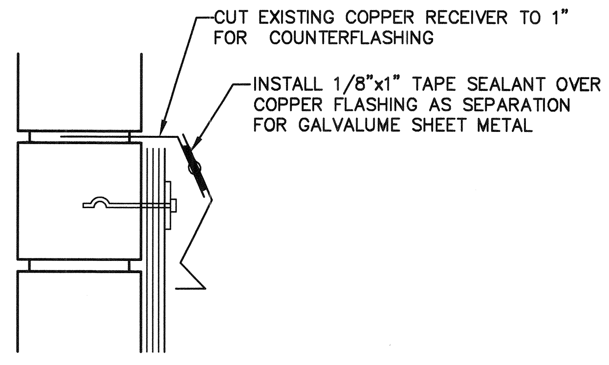
DETAIL P NTS
