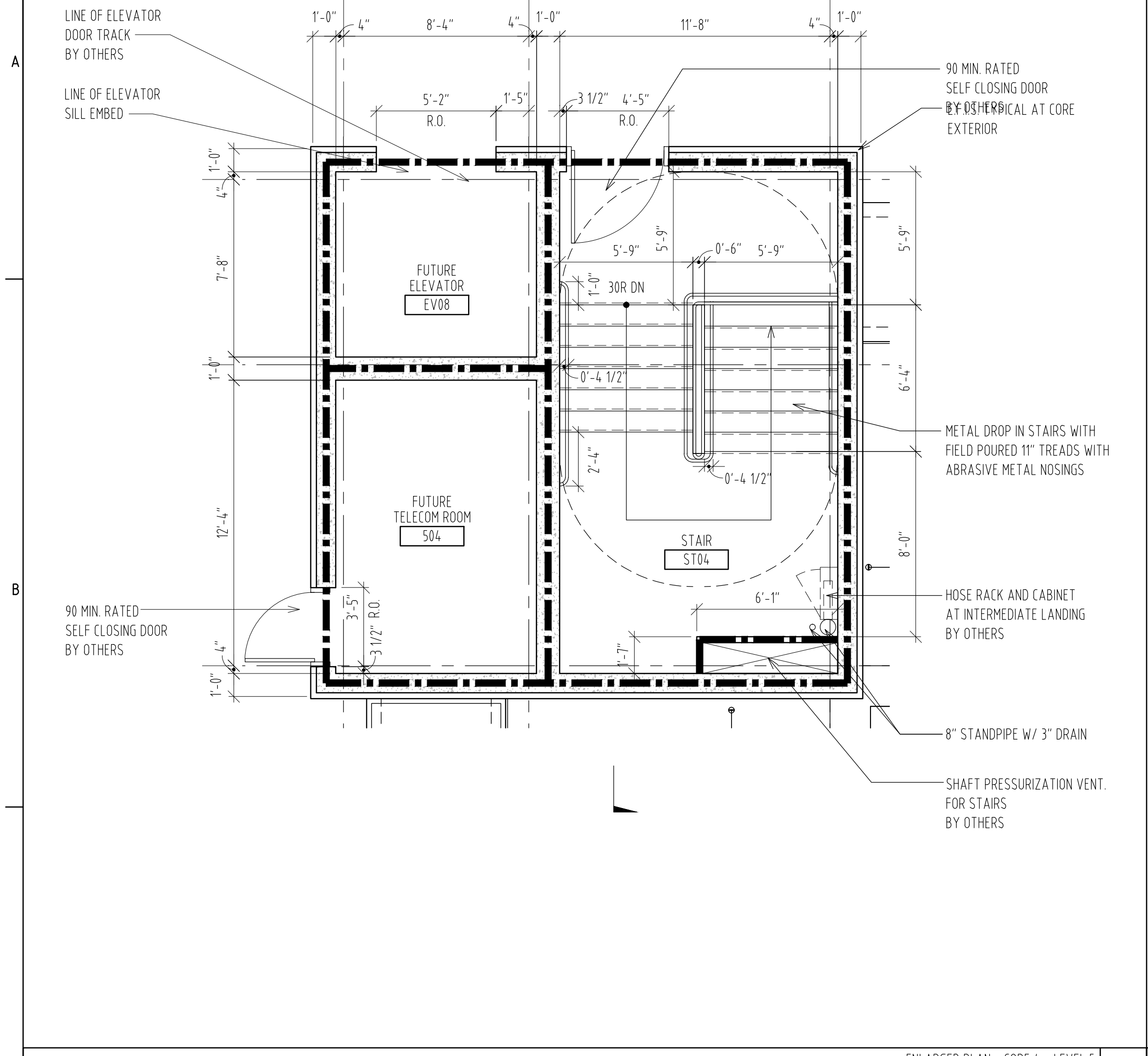
ENLARGED PLAN - CORE 4 - LEVEL 5 SCALE: 1/4" = 1'-0"
