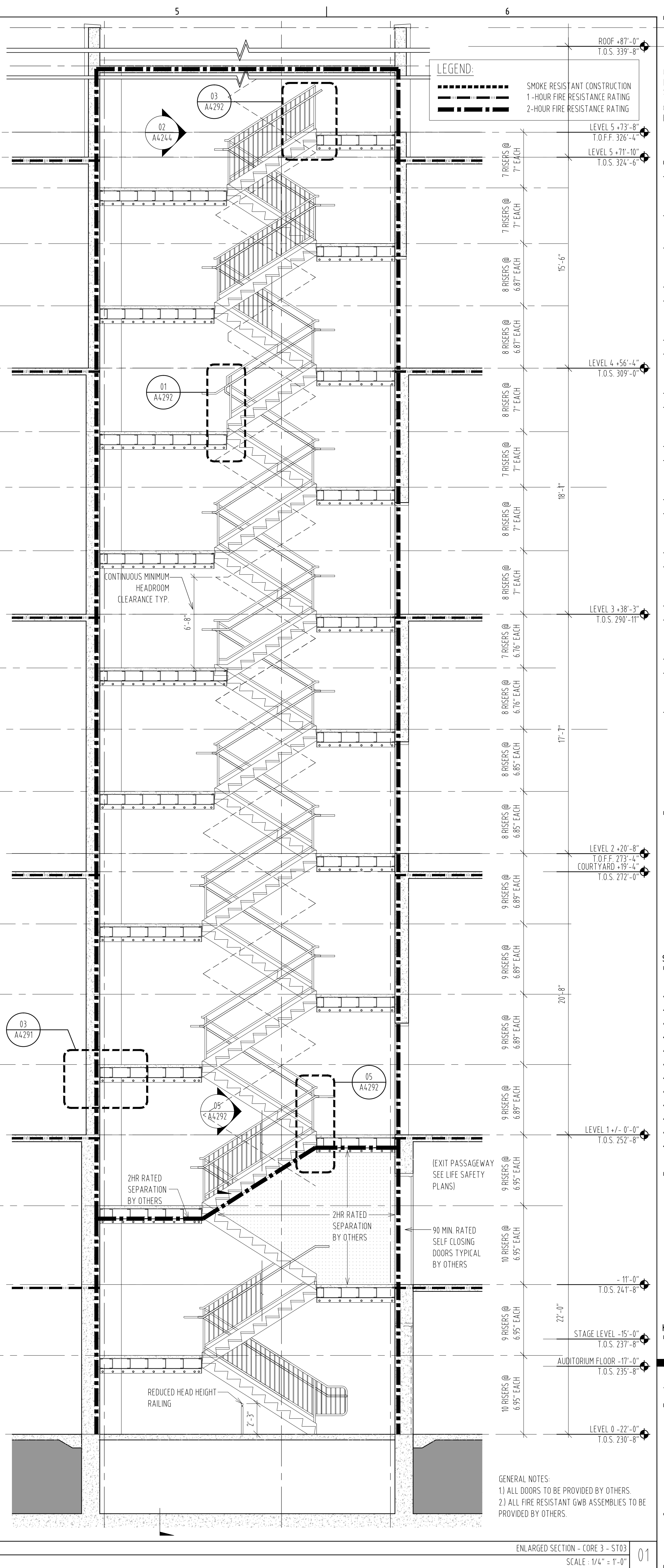
ENLARGED SECTION - CORE 3 SCALE: 1/4" = 1'-0"
