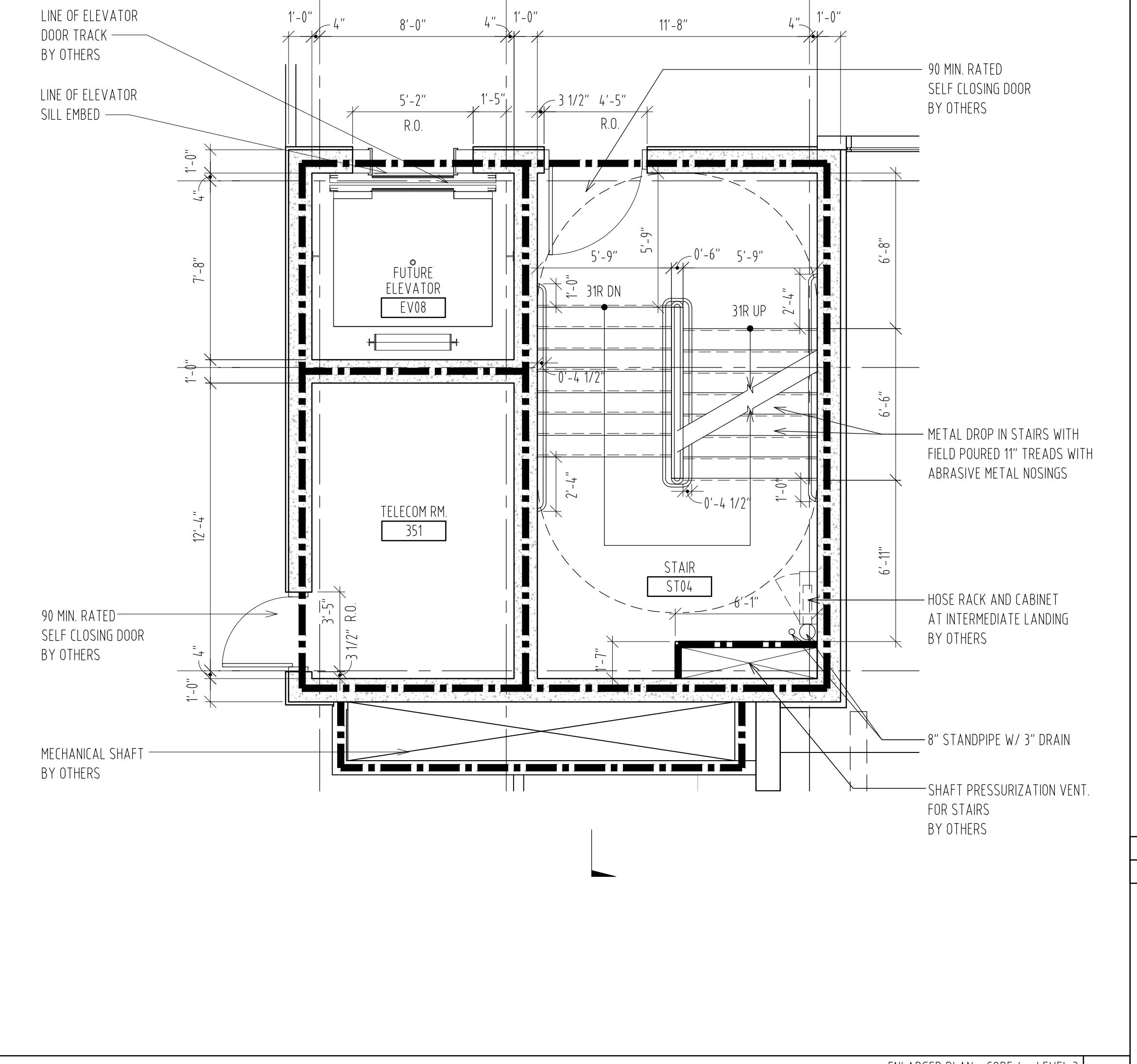
ENLARGED PLAN - CORE 4 - LEVEL 3 SCALE: 1/4" = 1'-0"
