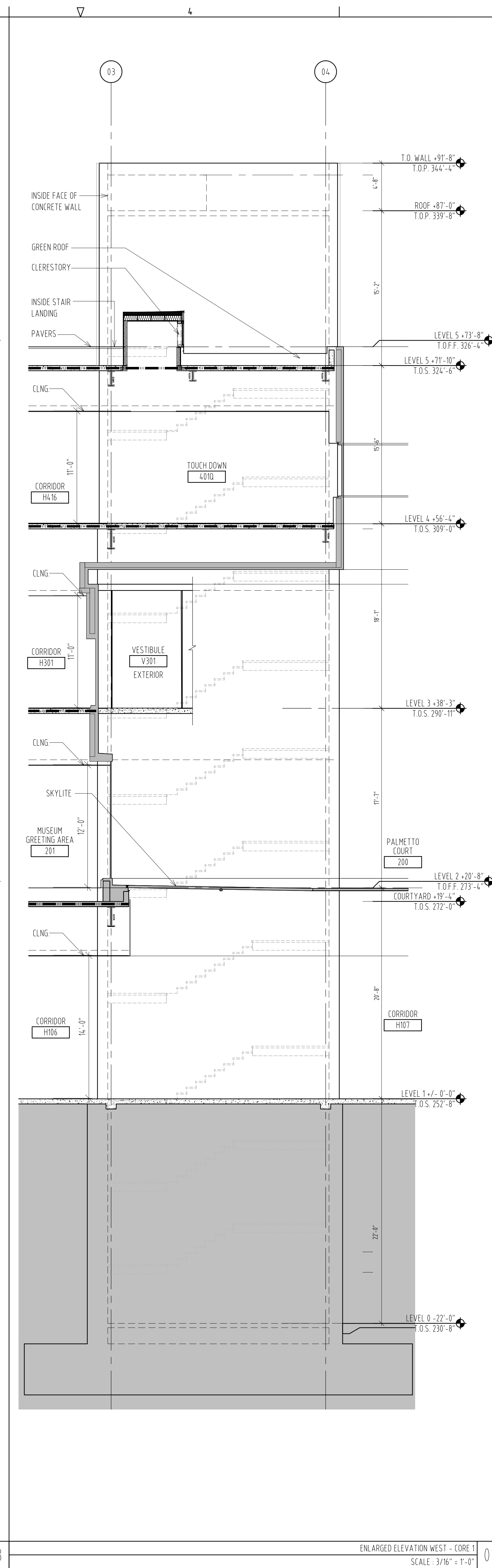
ENLARGED ELEVATION NORTH - CORE 1 SCALE: 3/16" = 1'-0"
