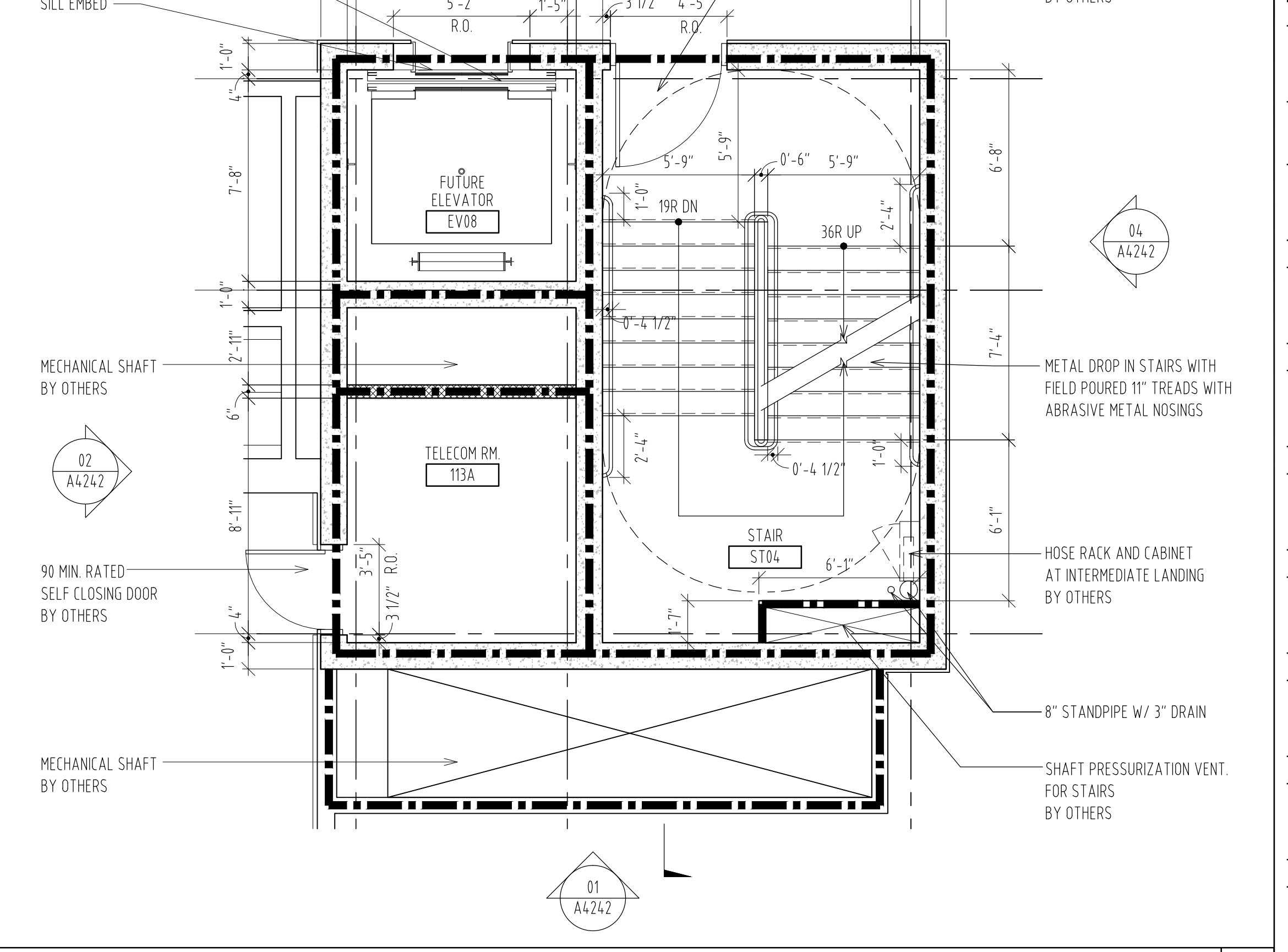
ENLARGED PLAN - CORE 4 - LEVEL 1 SCALE: 1/4" = 1'-0"
