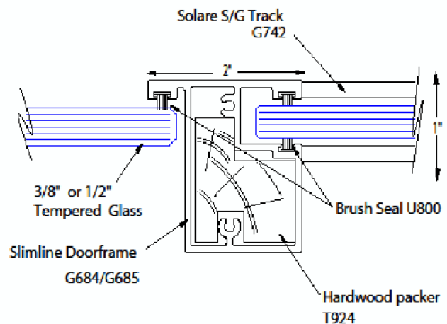
Slimline Doorframe Detail (Glass Door)
