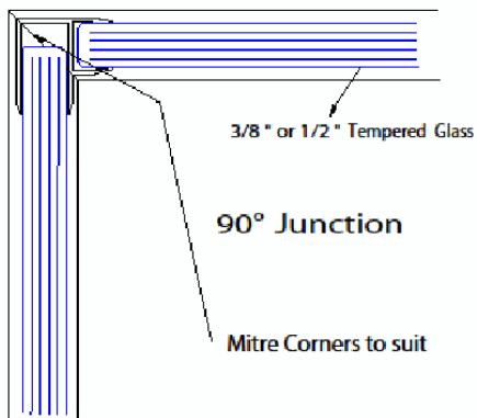
Single Glazed Corner Details
