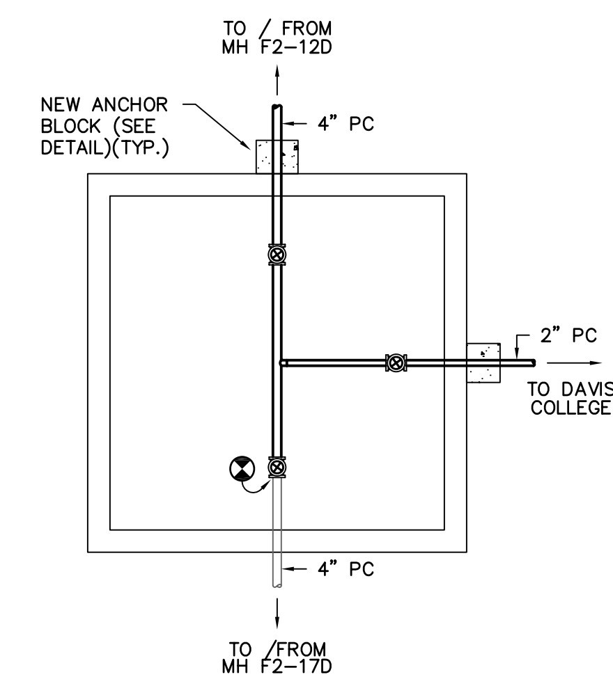
3 VAULT F2-18D NO SCALE
