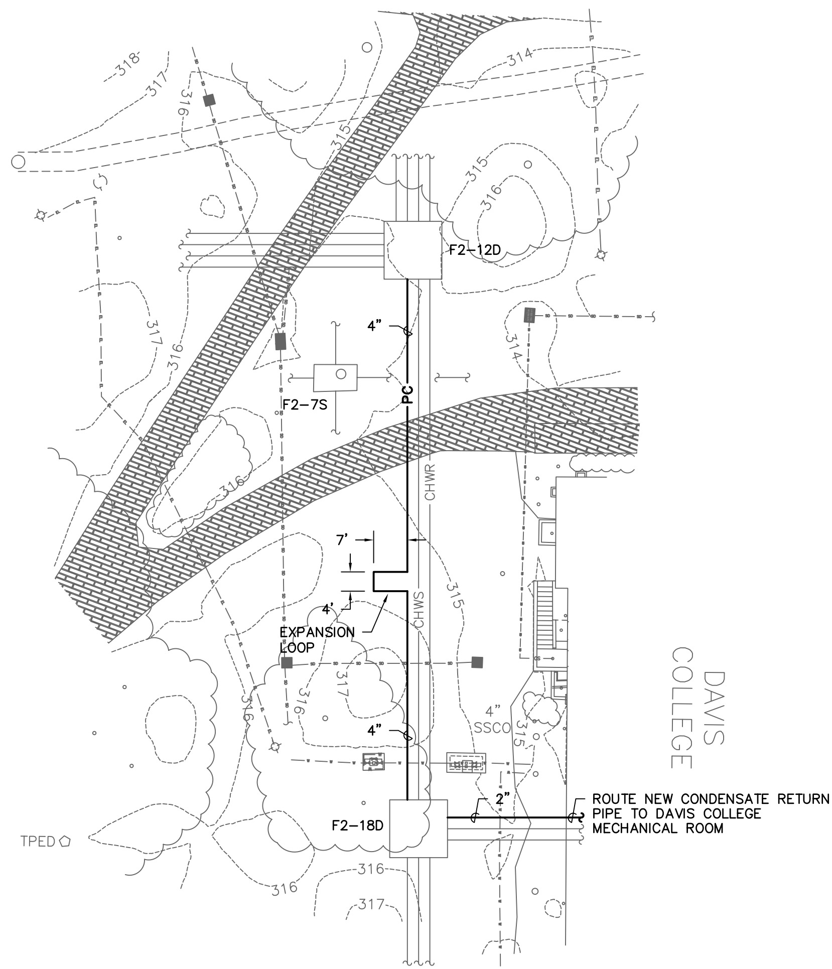
1 SITE PLAN - RENOVATION SCALE: 1" = 20'
