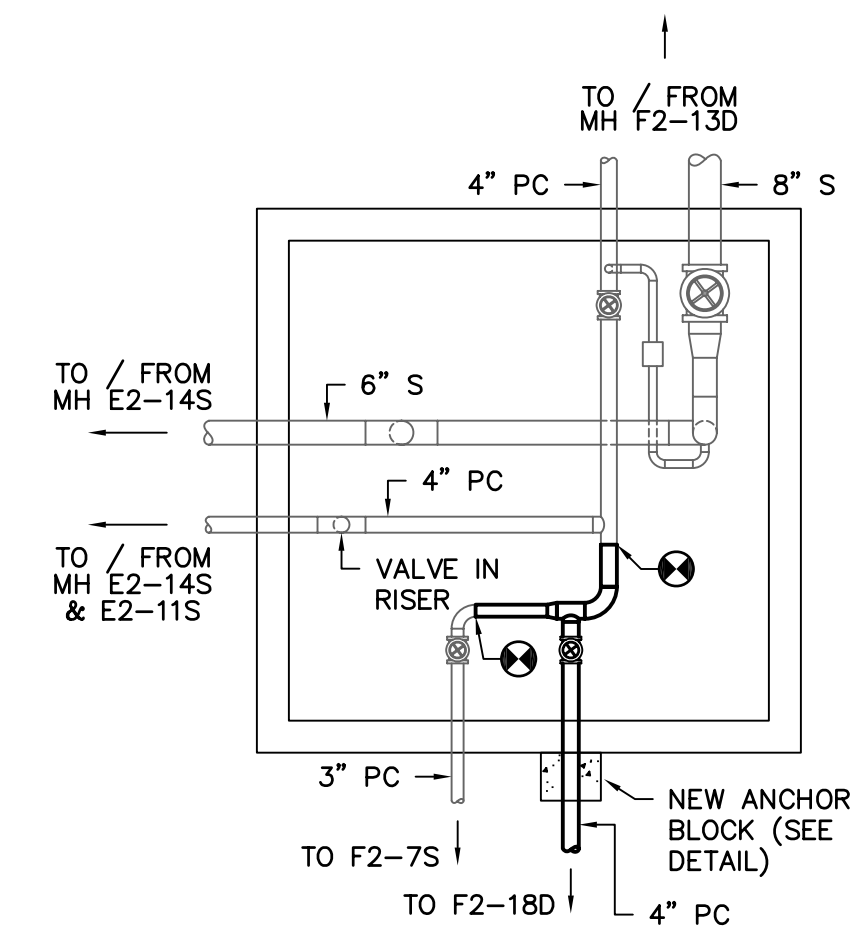
2 VAULT F2-12D NO SCALE
