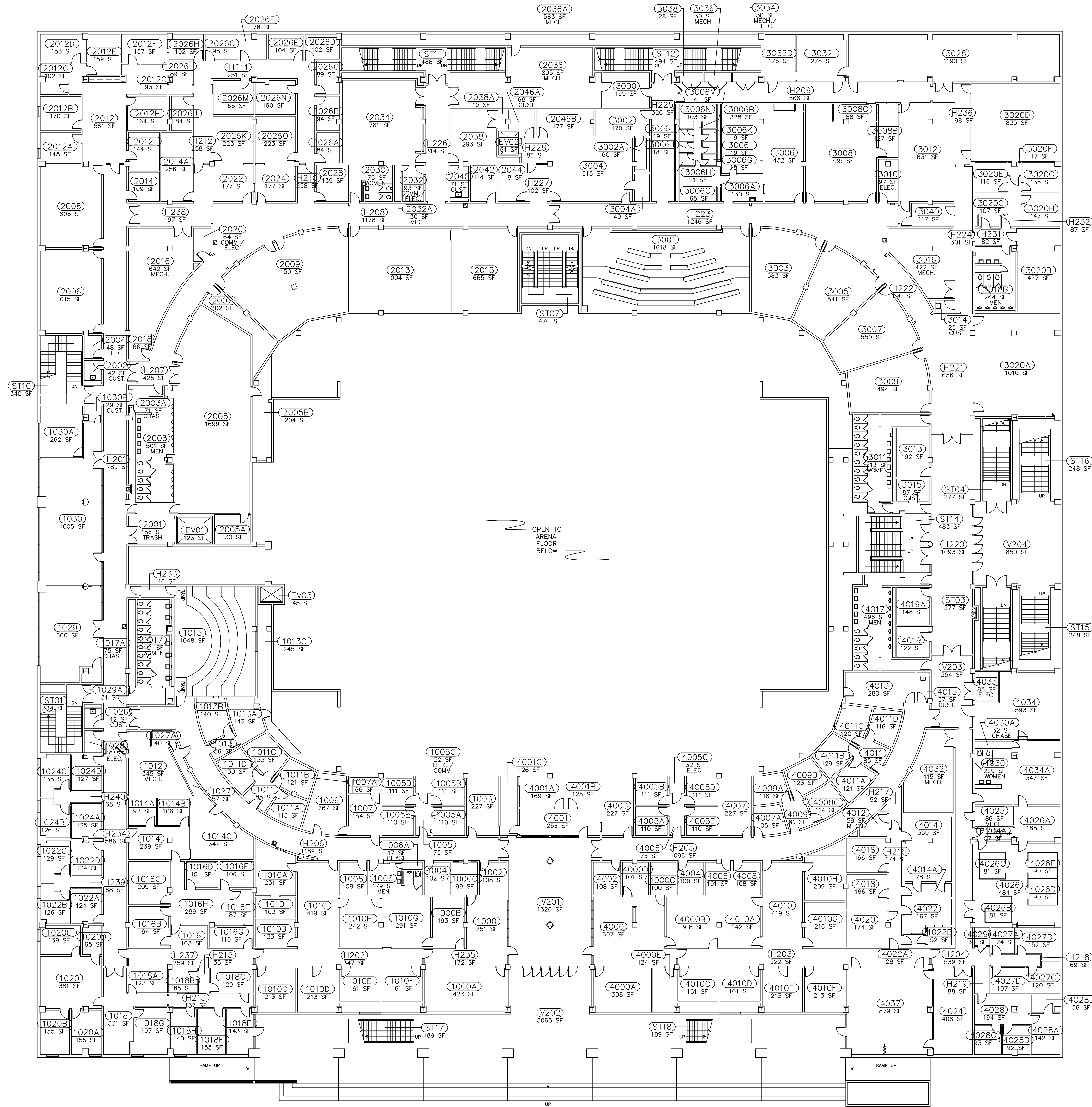
N 1 A2 ACADEMIC LEVEL SECOND FLOOR PLAN - 084 SCALE: 1/16" = 1'-0"
